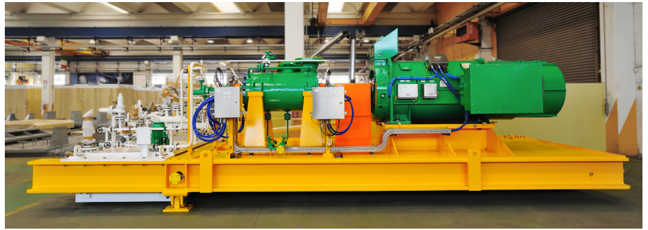
BB5 AHPB pump skid equipped with lube oil and three points gimbal for floating unit installations
